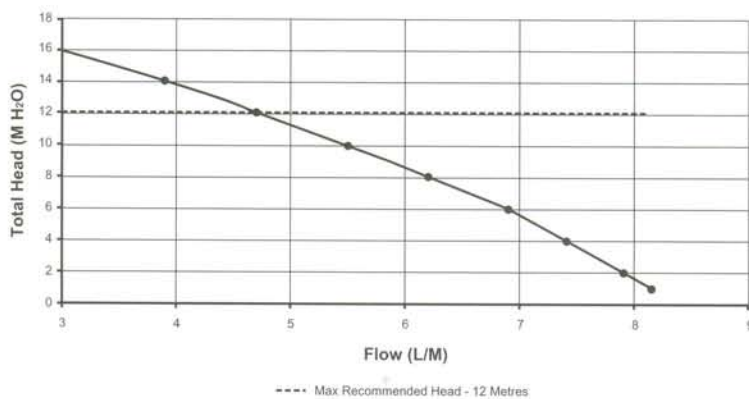
Flow Rate - 230V Motor
